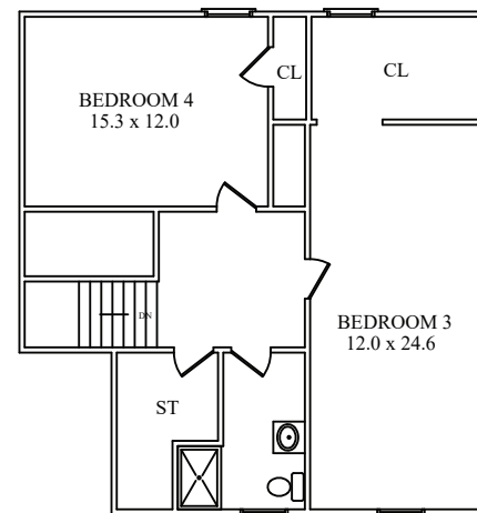
THIRD FLOOR
