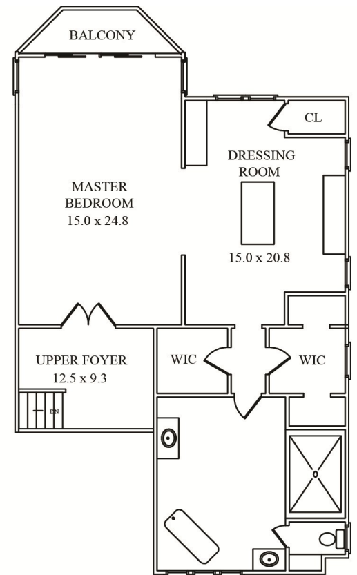
THIRD LEVEL
