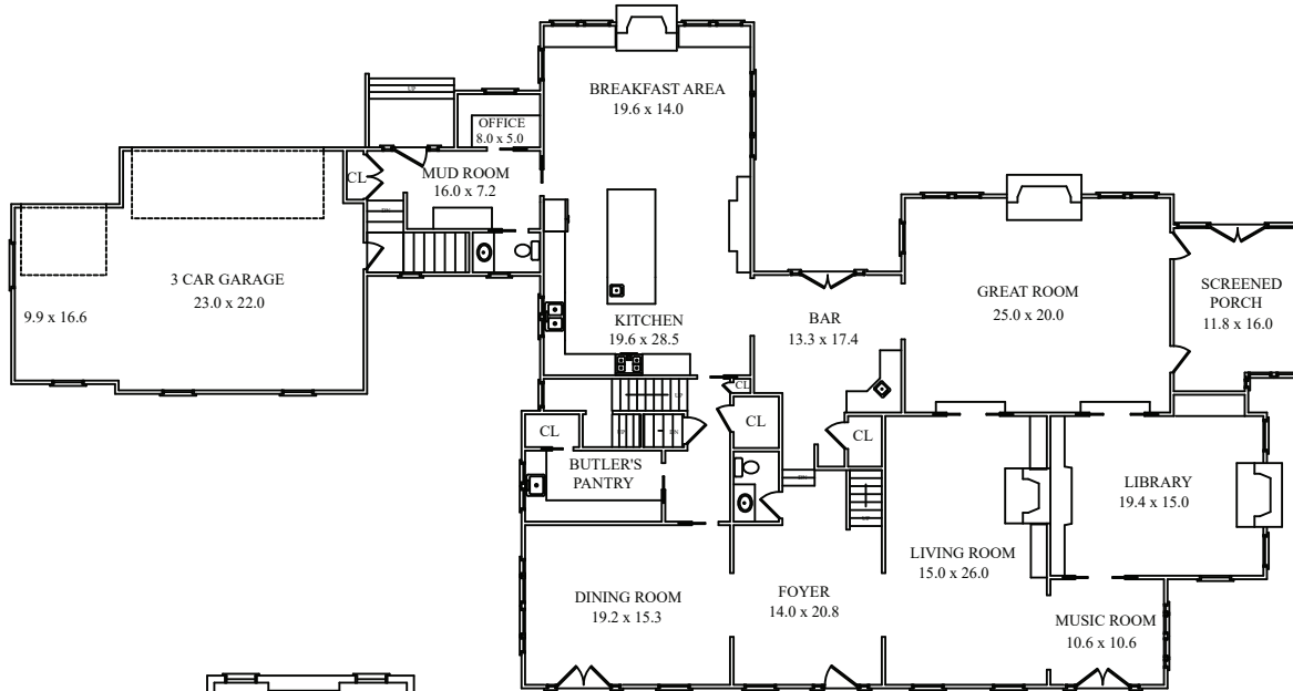
FIRST FLOOR
