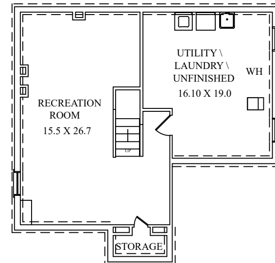
LOWER LEVEL
