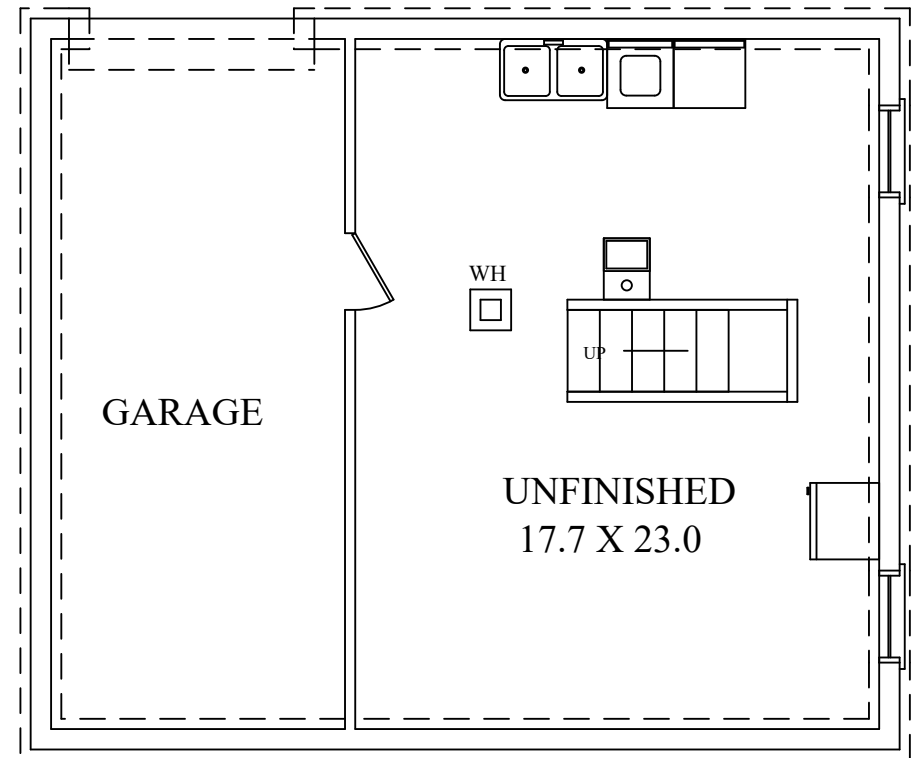
LOWER LEVEL
