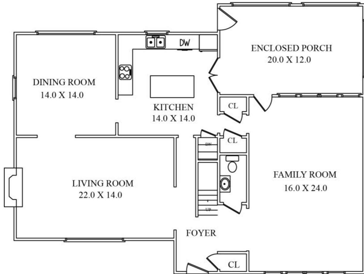
FIRST LEVEL
