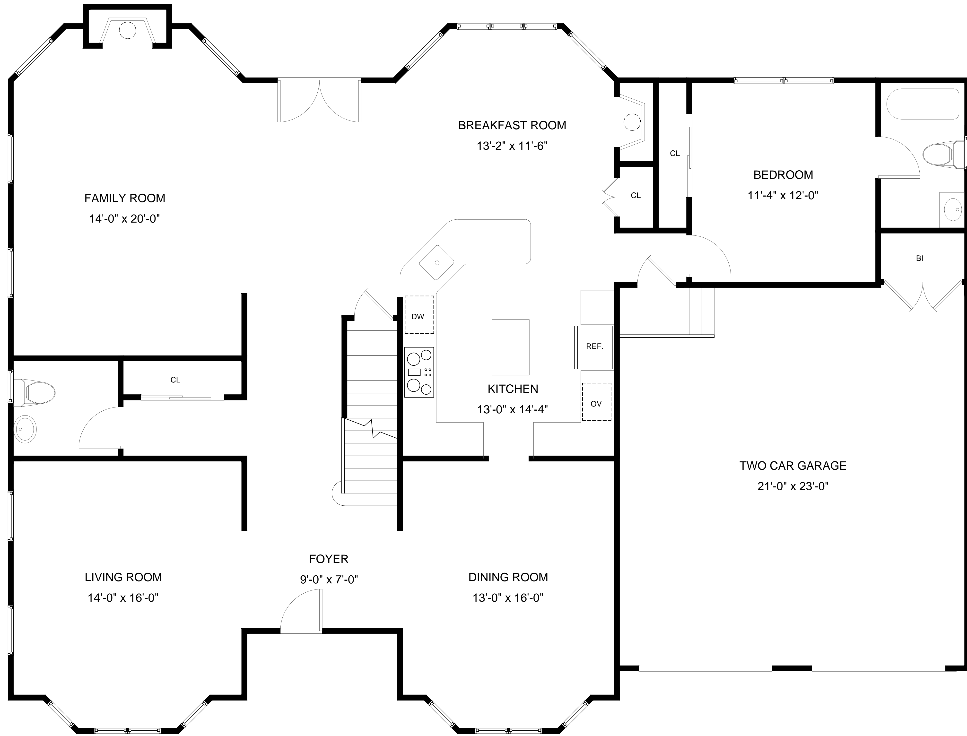
FIRST FLOOR
