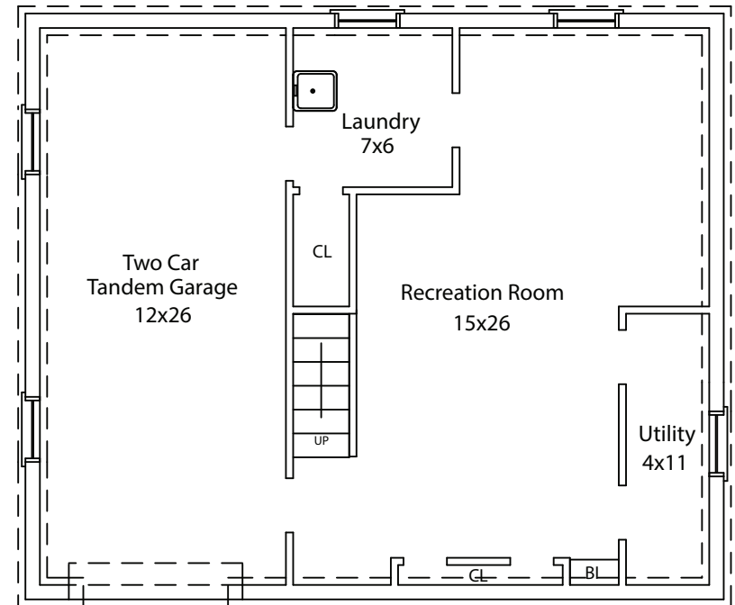
BASEMENT
