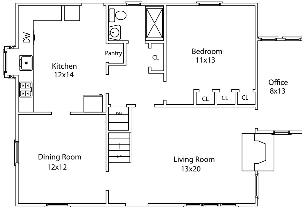
FIRST FLOOR
