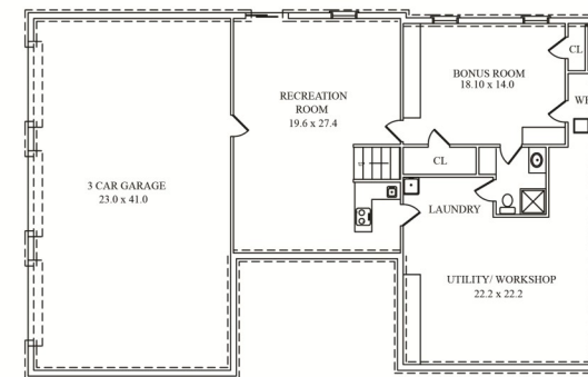
LOWER LEVEL
