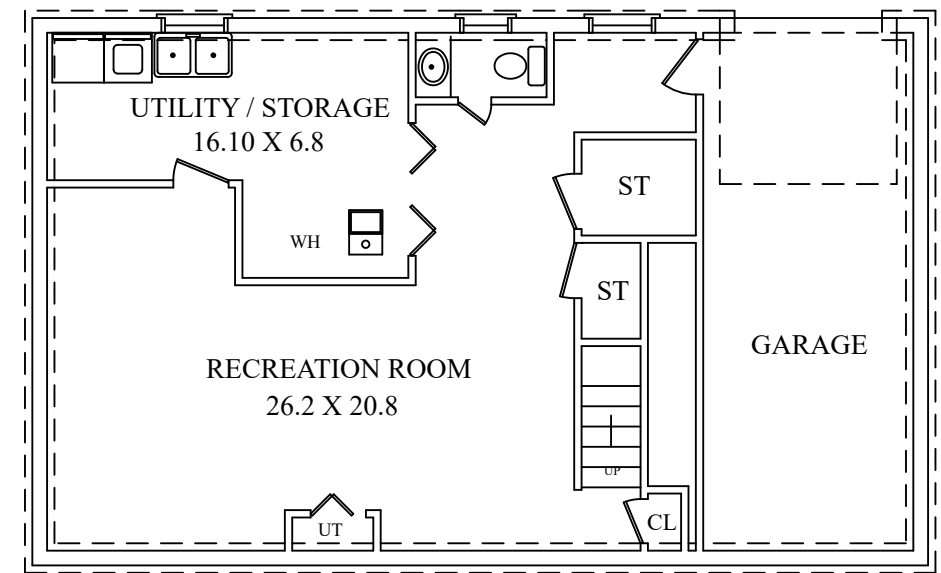
LOWER LEVEL
