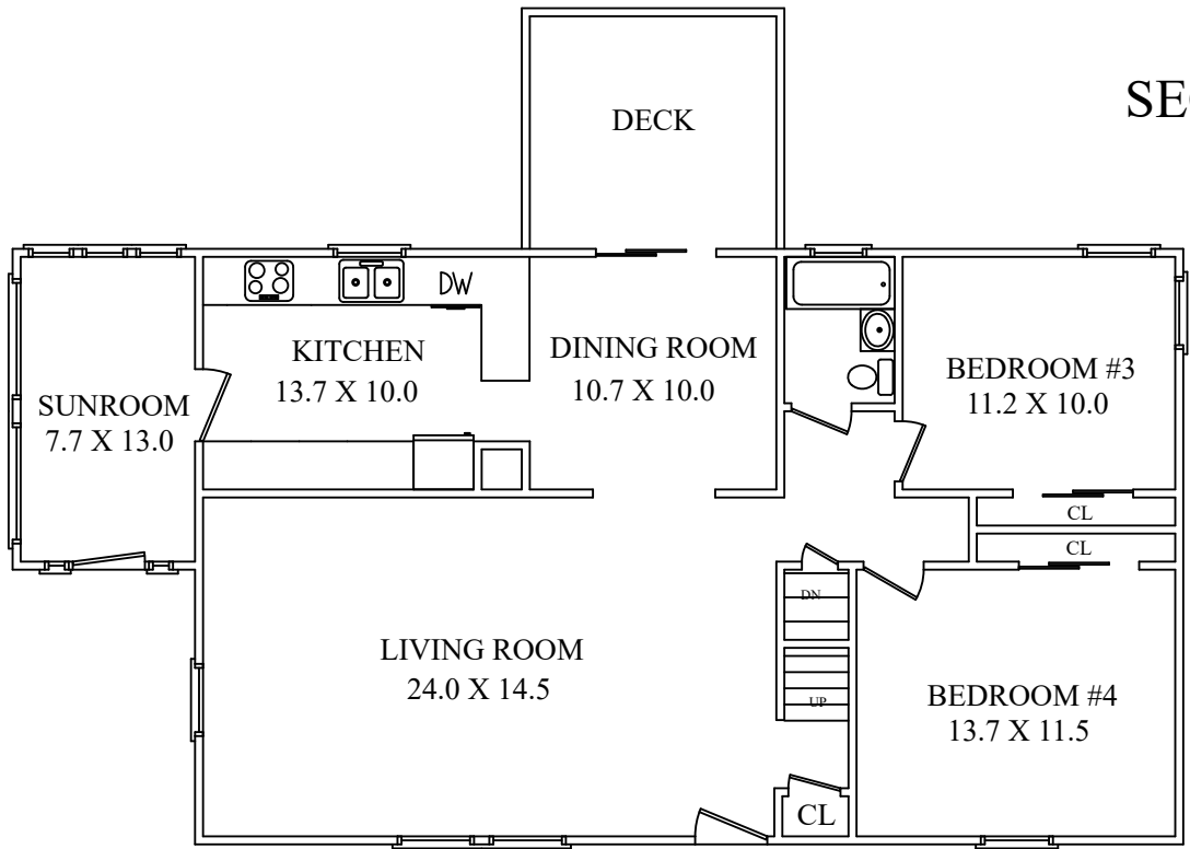
FIRST FLOOR
