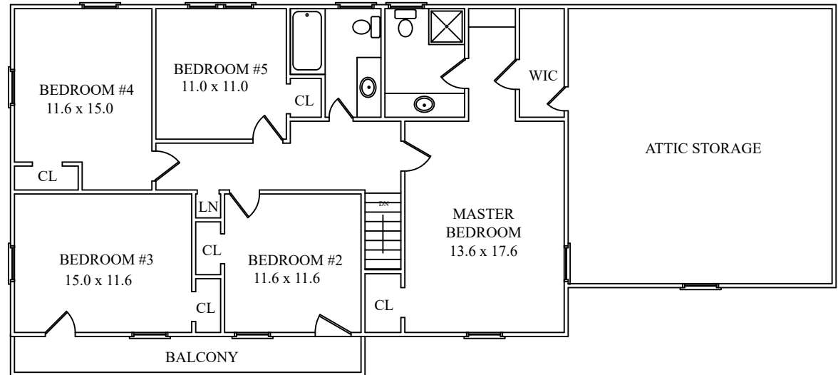
SECOND FLOOR
