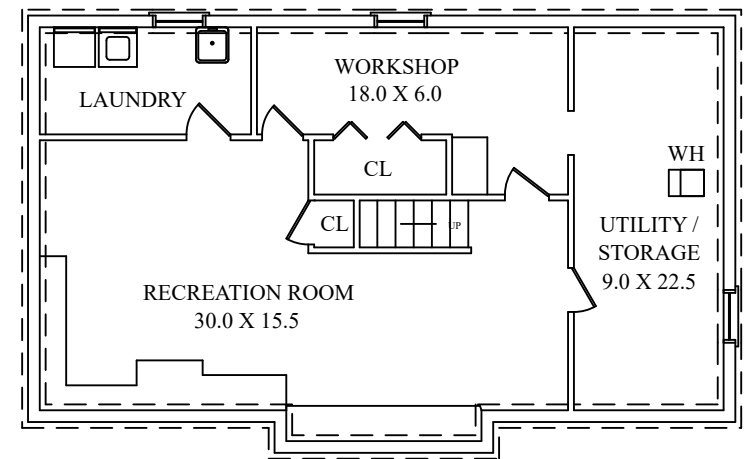
LOWER LEVEL
