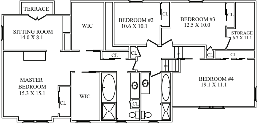
THIRD FLOOR
