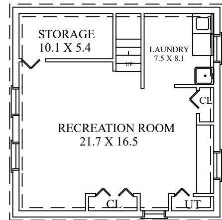
LOWER LEVEL
