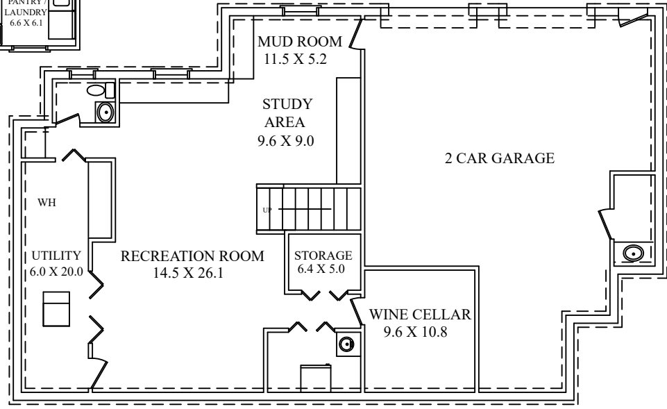
LOWER LEVEL
