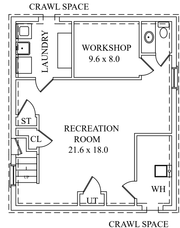
LOWER LEVEL
