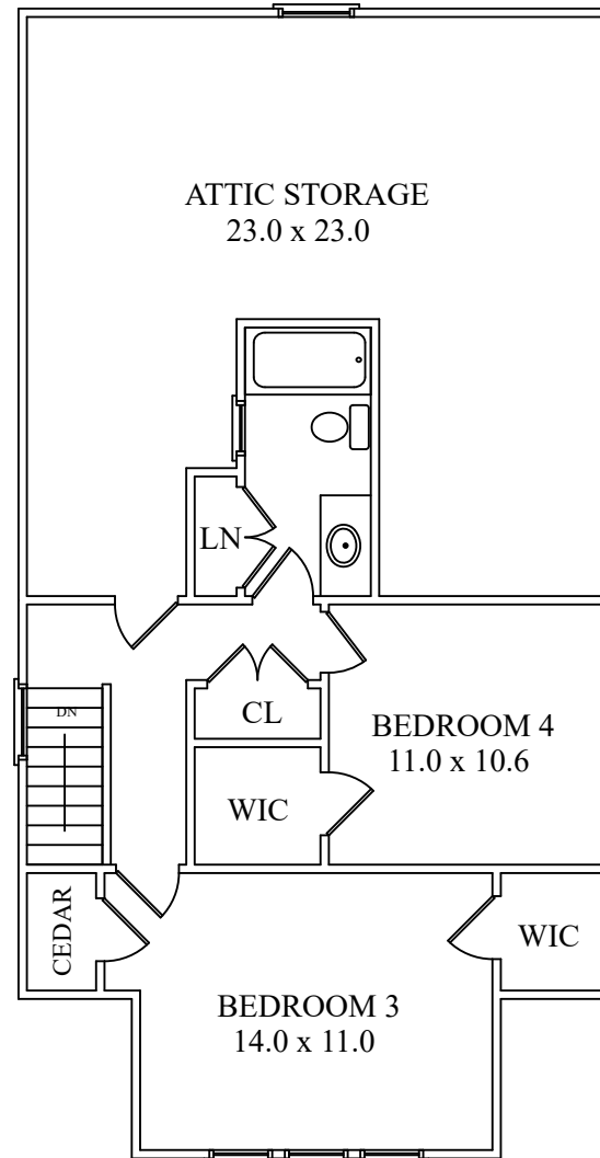
SECOND FLOOR
