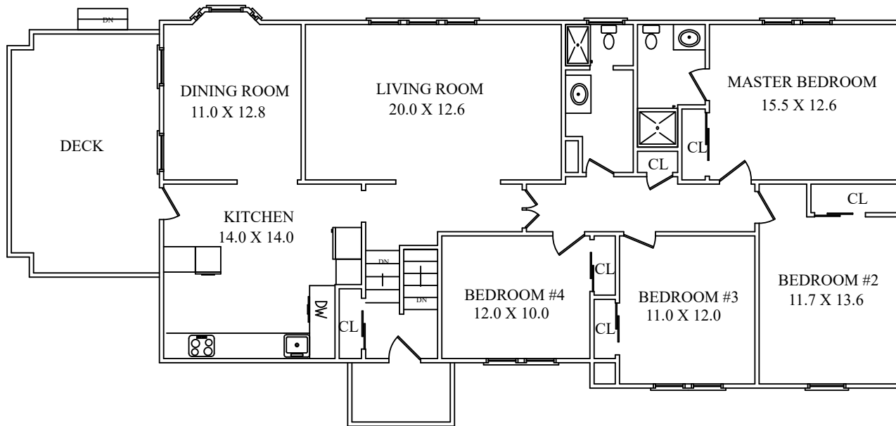
FIRST FLOOR
