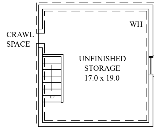
LOWER LEVEL
