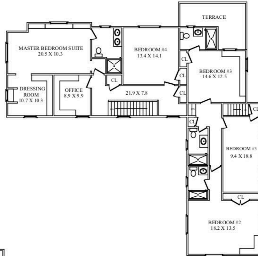
SECOND LEVEL
