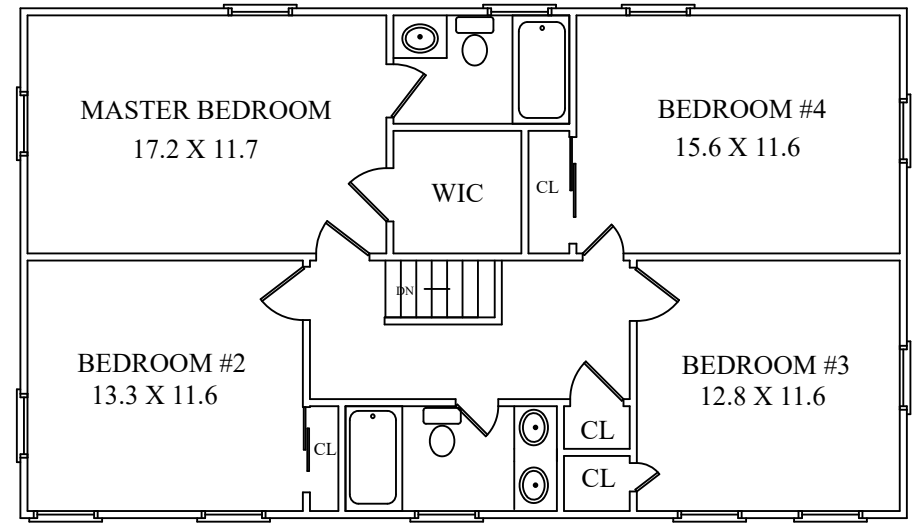
SECOND FLOOR
