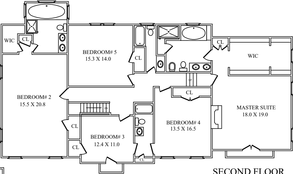
SECOND FLOOR
