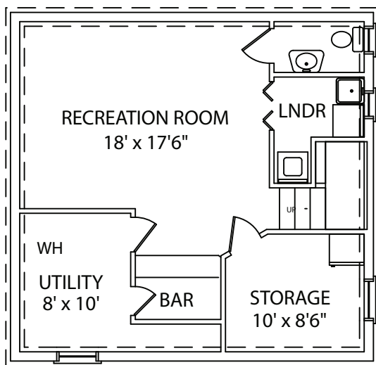
LOWER LEVEL
