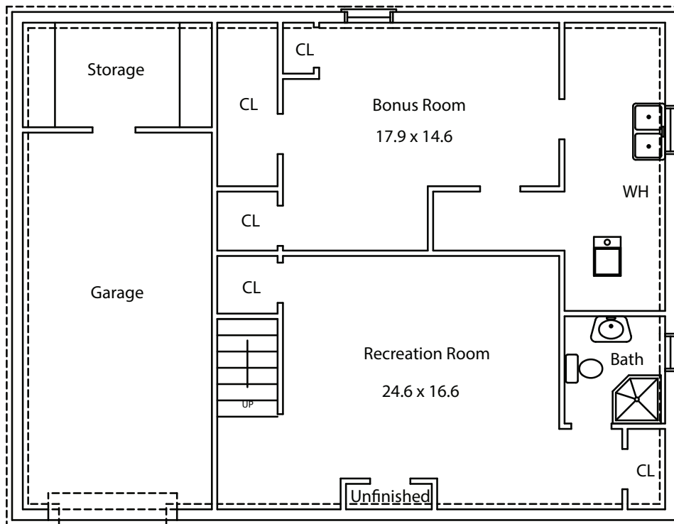
LOWER LEVEL
