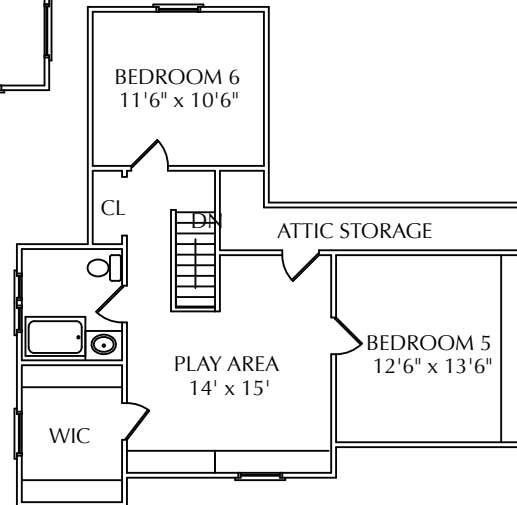
THIRD FLOOR
