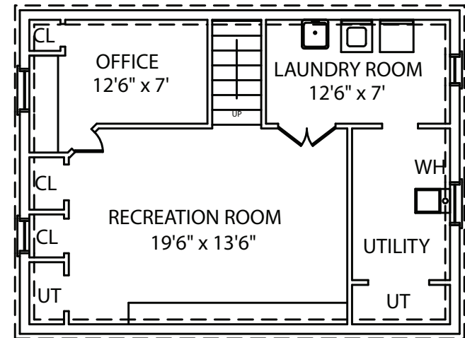
LOWER LEVEL
