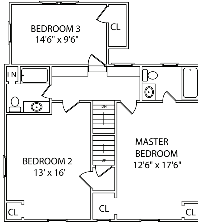
SECOND FLOOR
