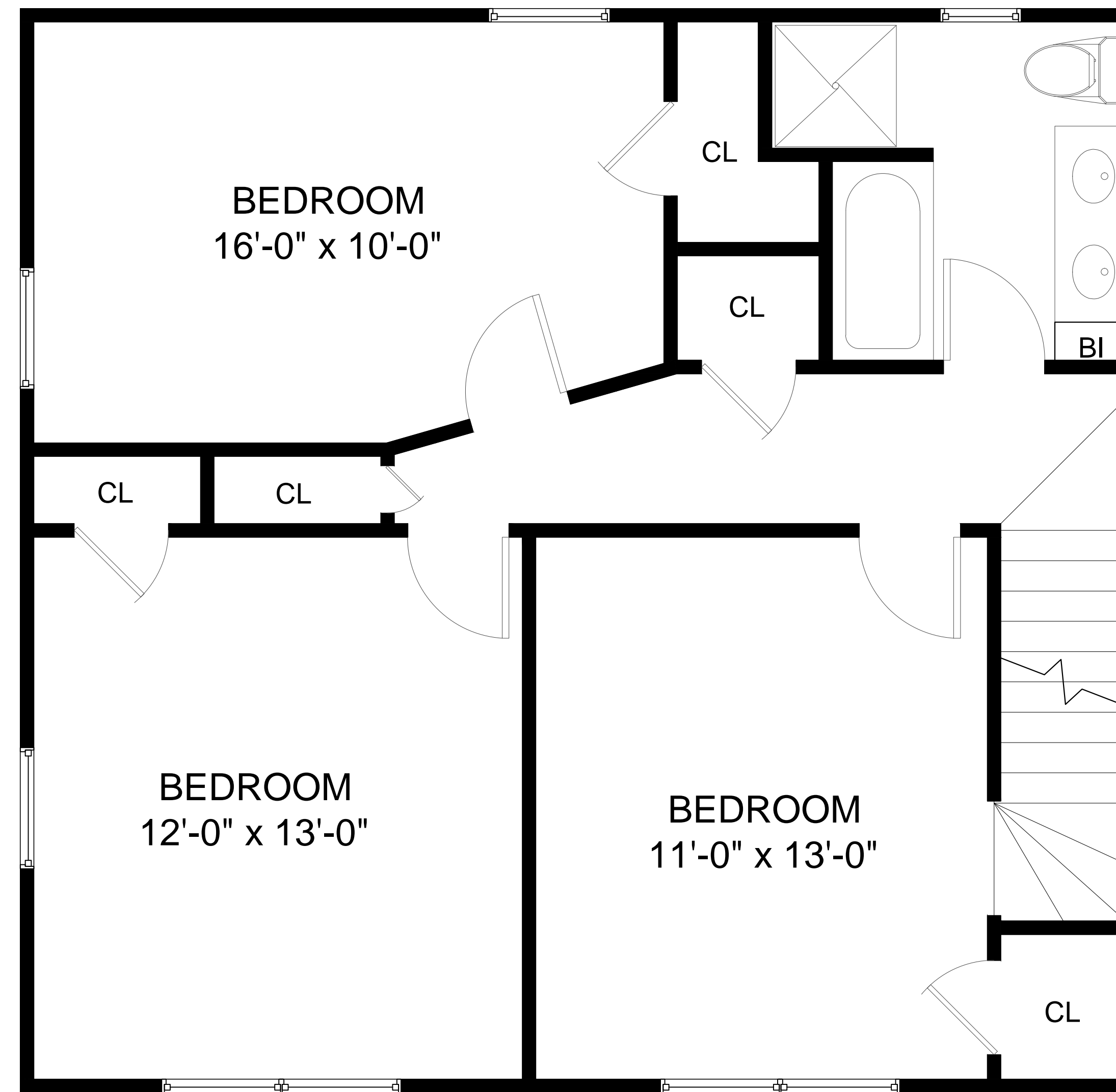
SECOND FLOOR
