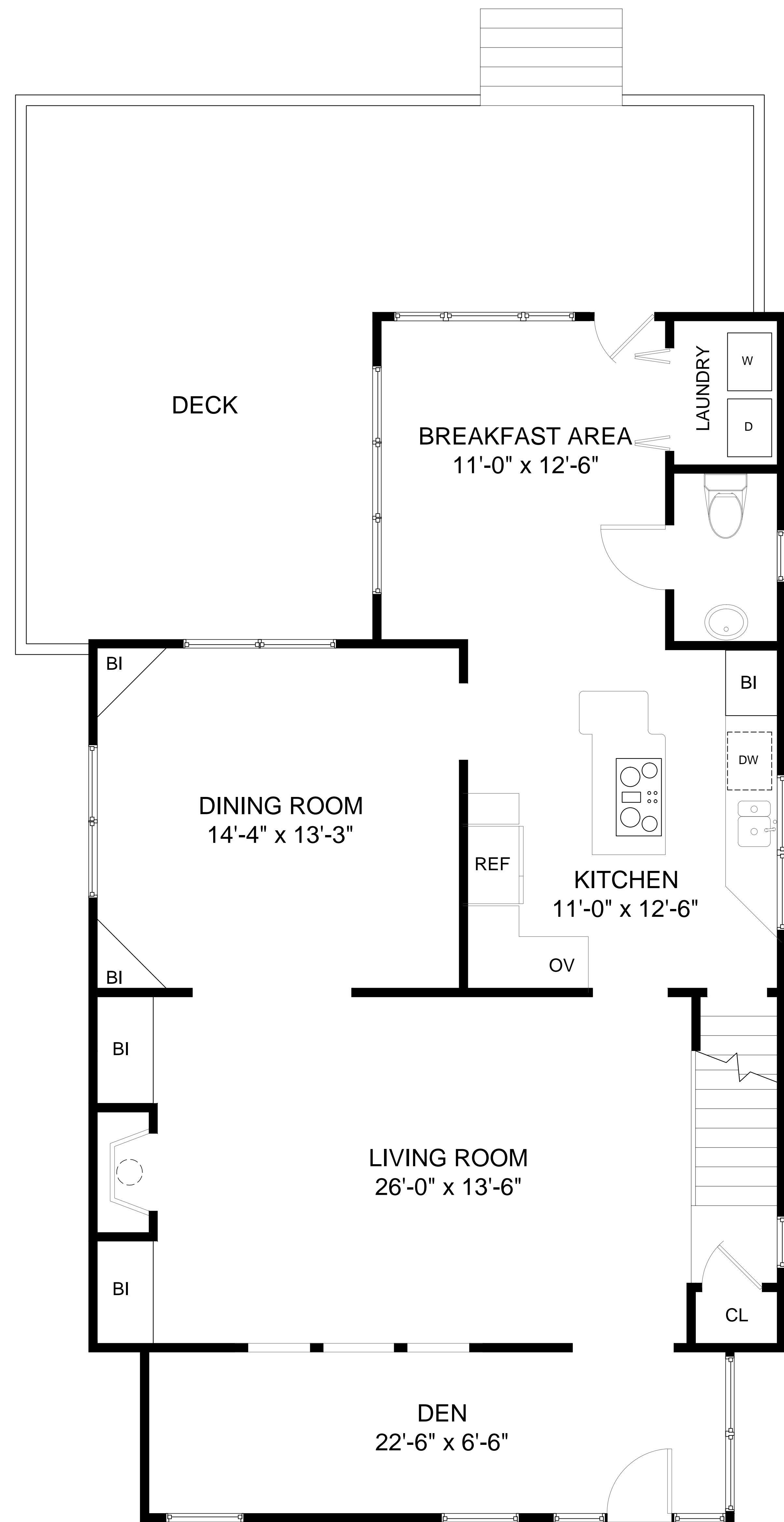
FIRST FLOOR
