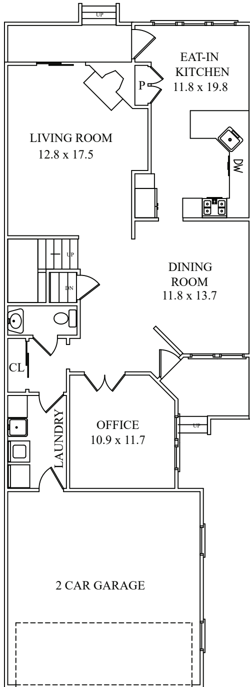
FIRST FLOOR
