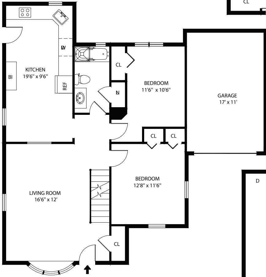
FIRST LEVEL (Approx. 990 SQ FT)
