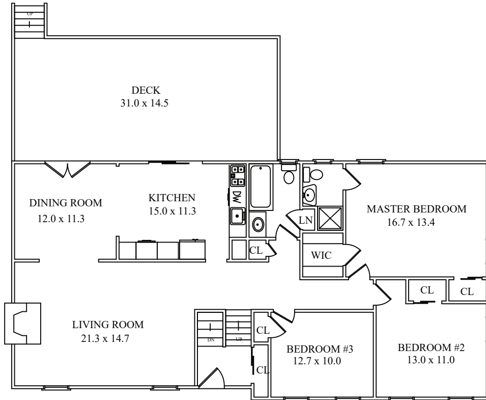
FIRST LEVEL
