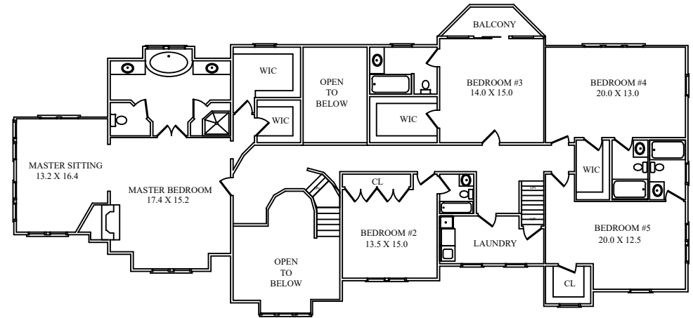
SECOND FLOOR
