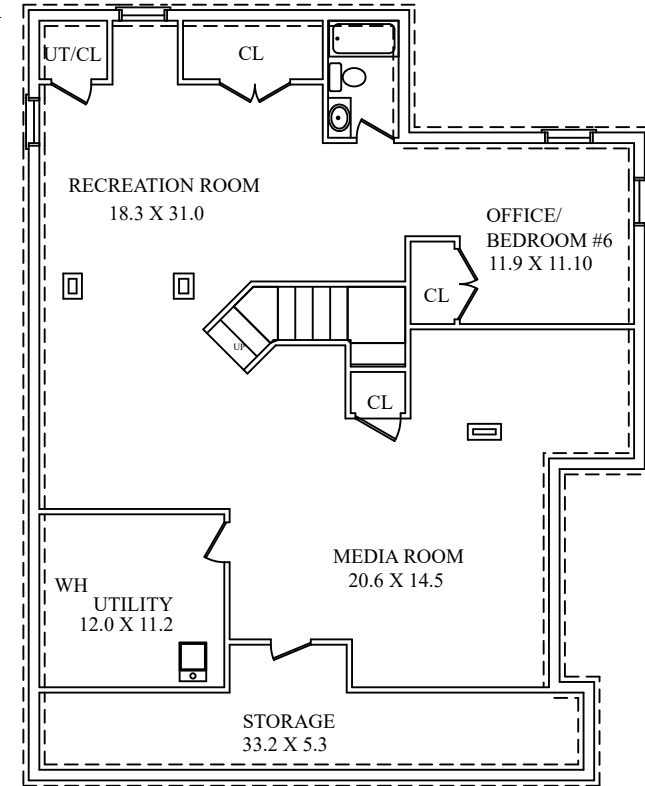
LOWER LEVEL
