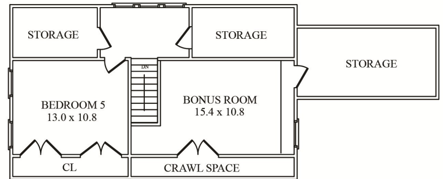
THIRD FLOOR
