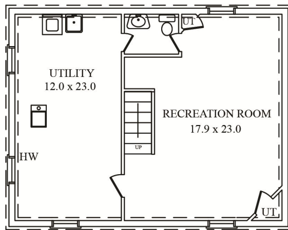
LOWER LEVEL
