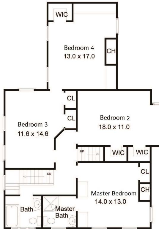
SECOND LEVEL
