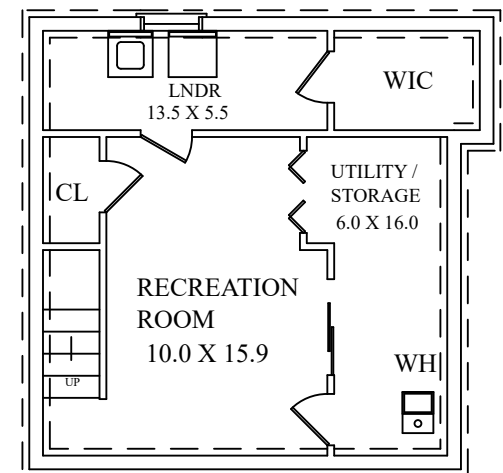
LOWER LEVEL
