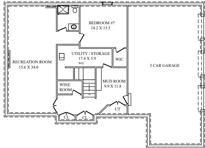
LOWER LEVEL
