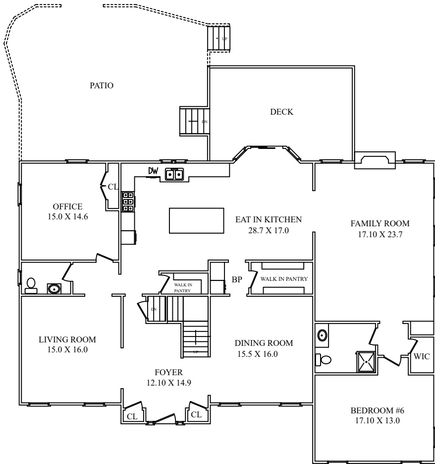
FIRST FLOOR
