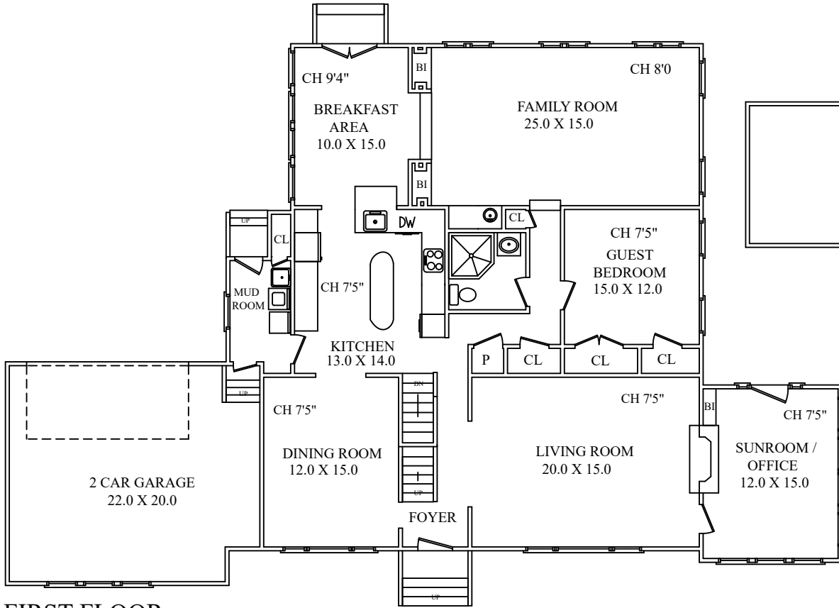
FIRST FLOOR
