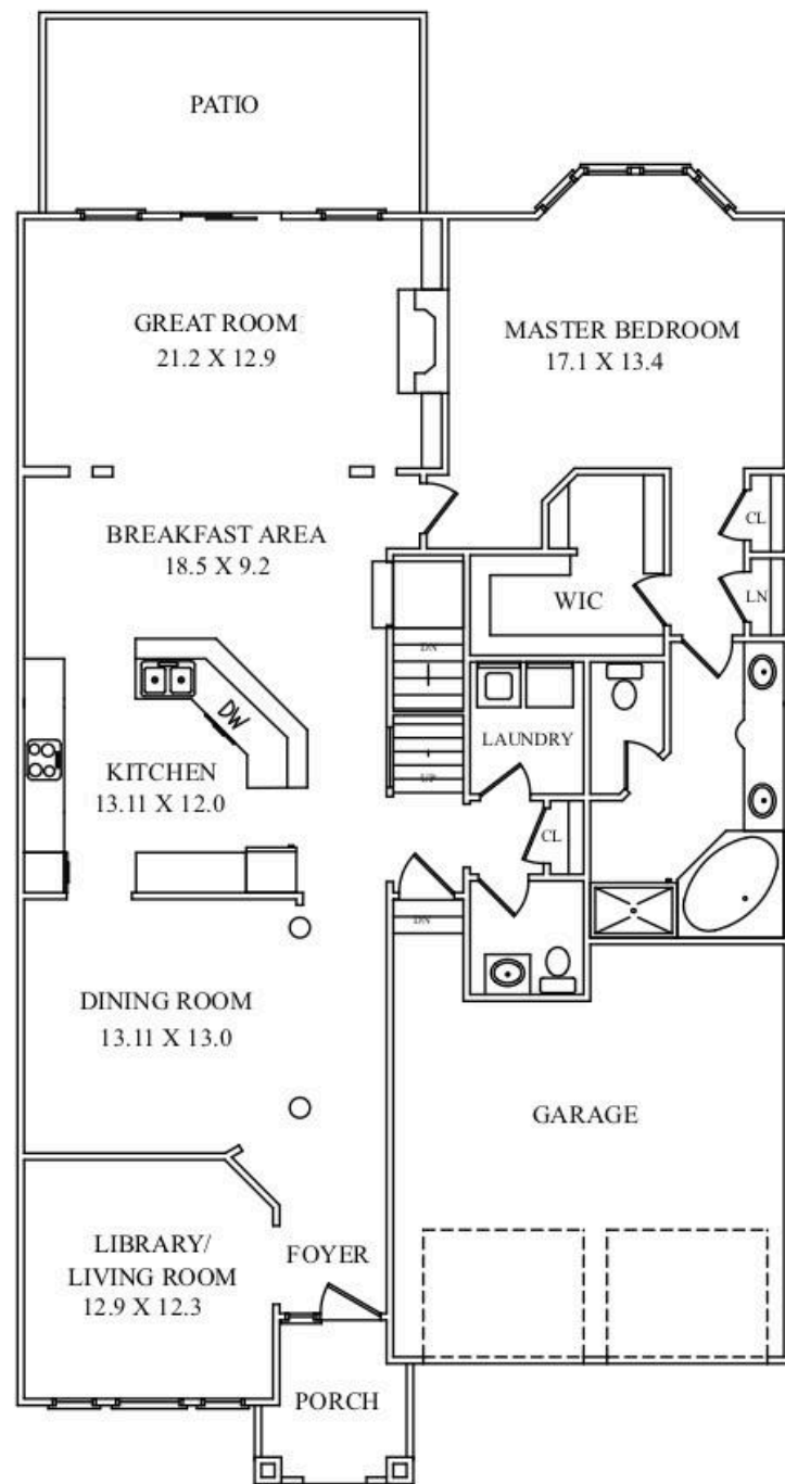
FIRST LEVEL
