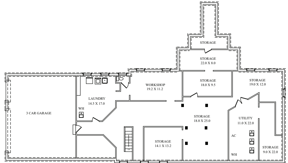
LOWER LEVEL
