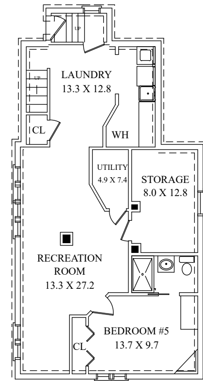
LOWER LEVEL
