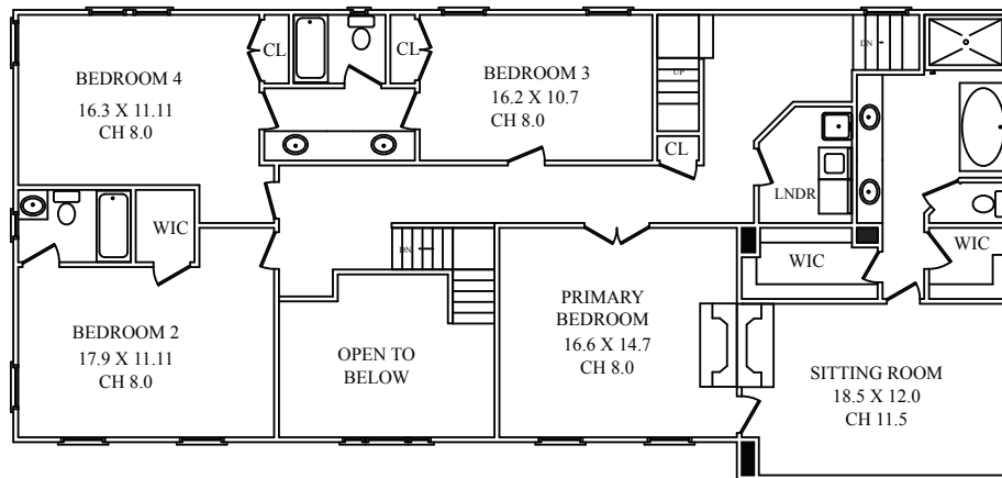
SECOND FLOOR
