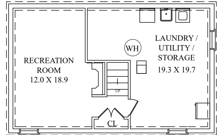
LOWER LEVEL
