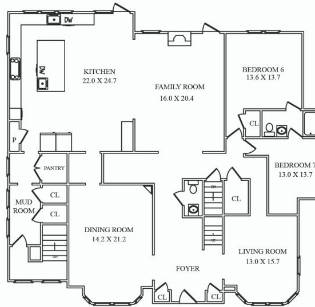
FIRST LEVEL
