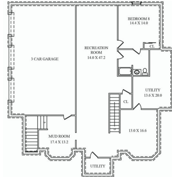
LOWER LEVEL
