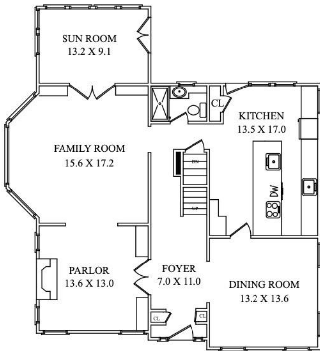
FIRST LEVEL
