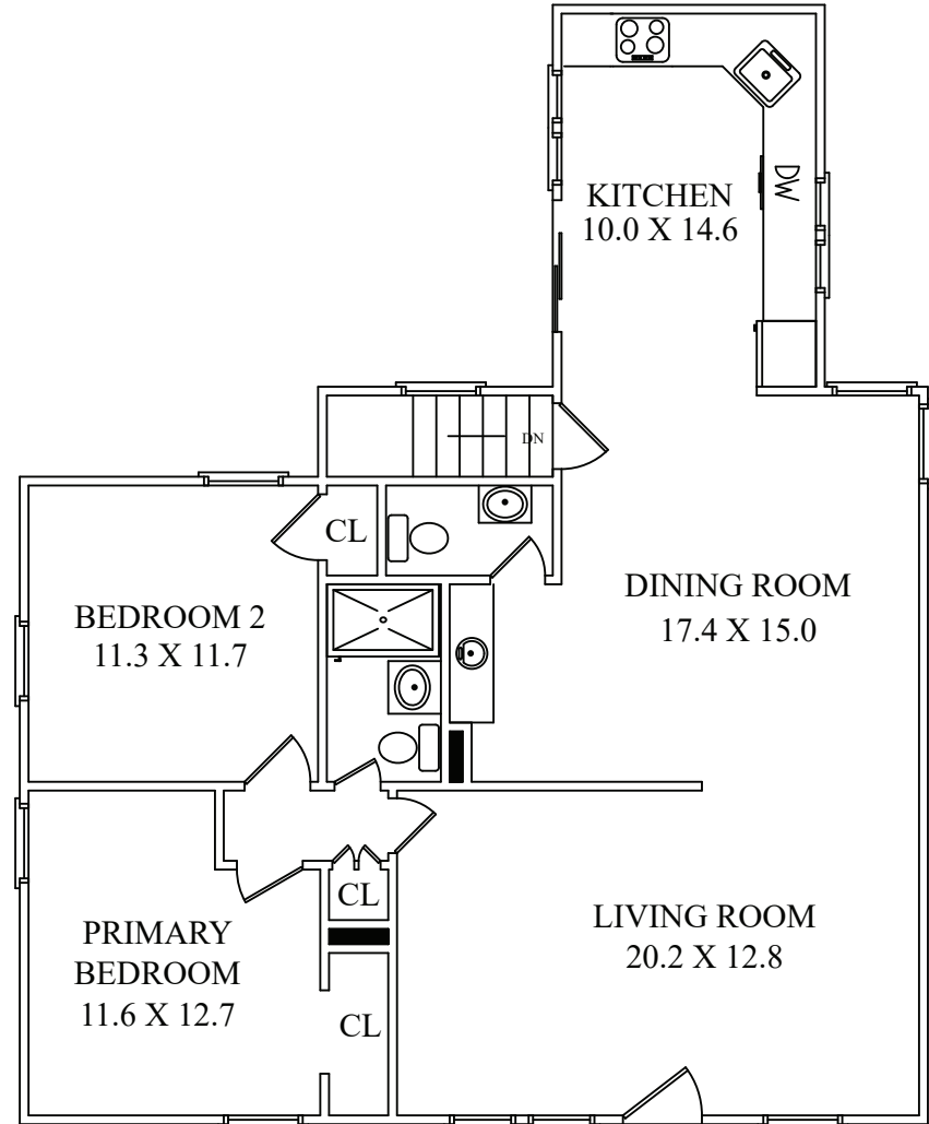
FIRST FLOOR
