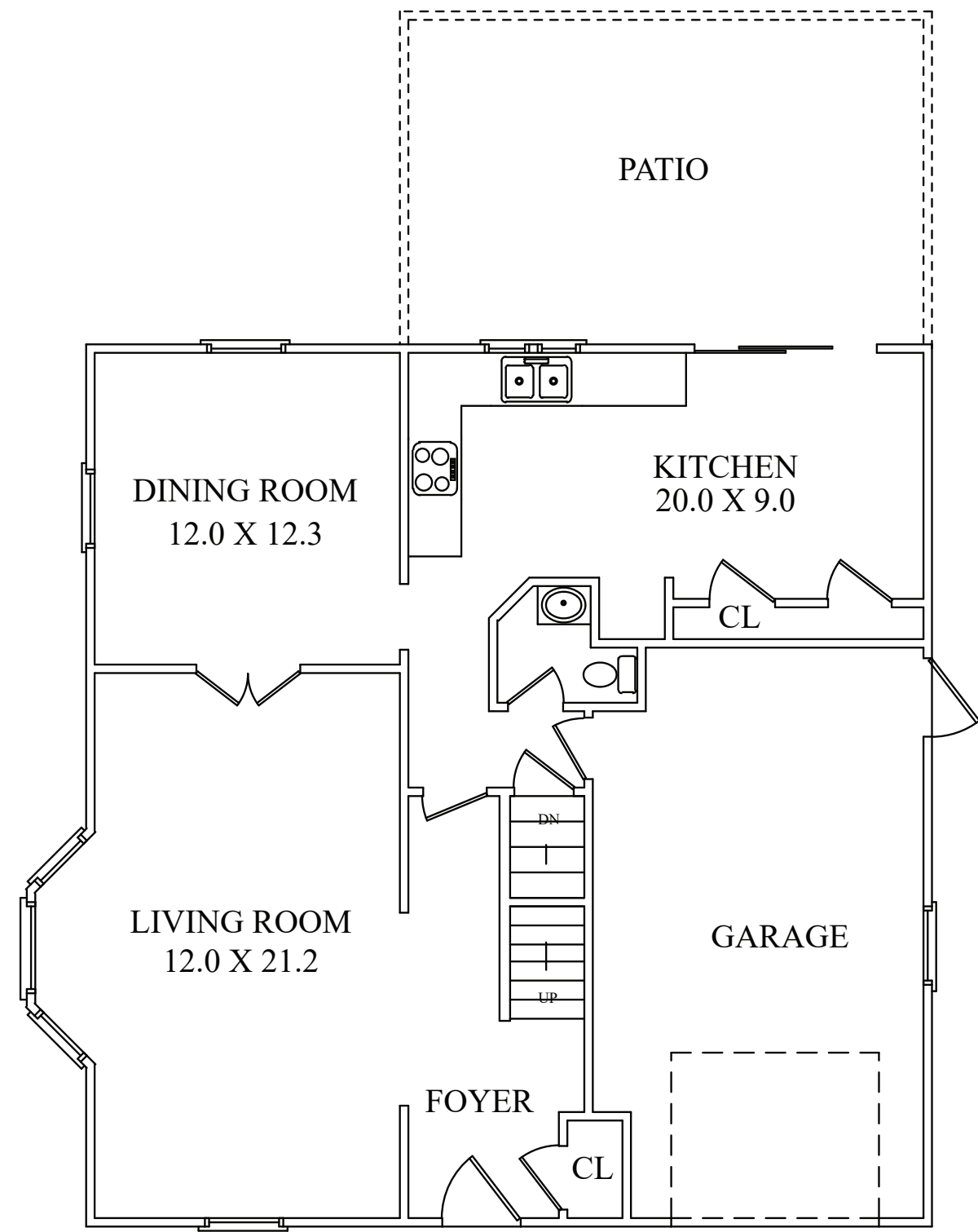
FIRST FLOOR
