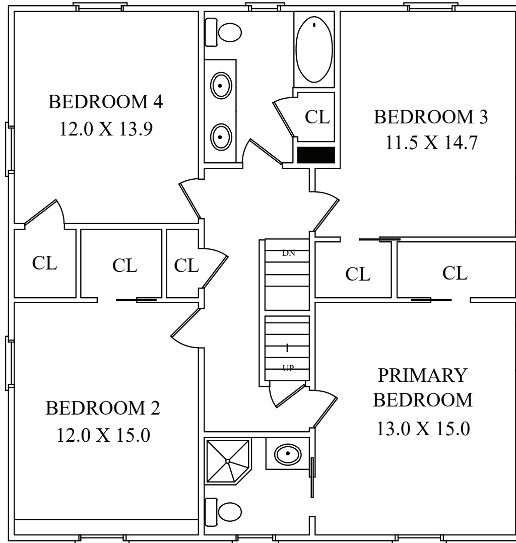
SECOND FLOOR
