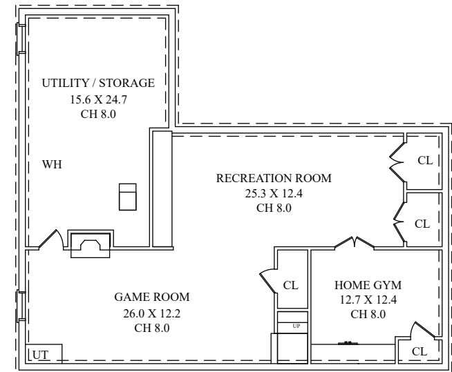
LOWER LEVEL
