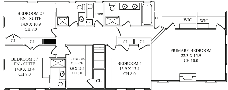
SECOND FLOOR
