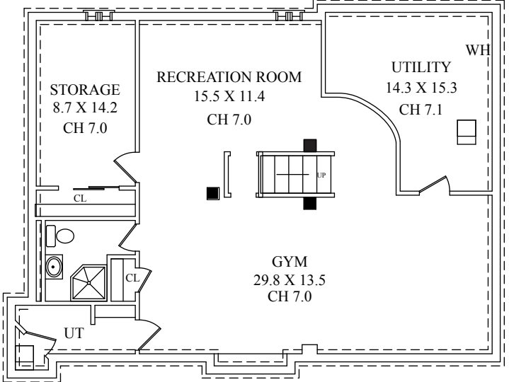
LOWER LEVEL
