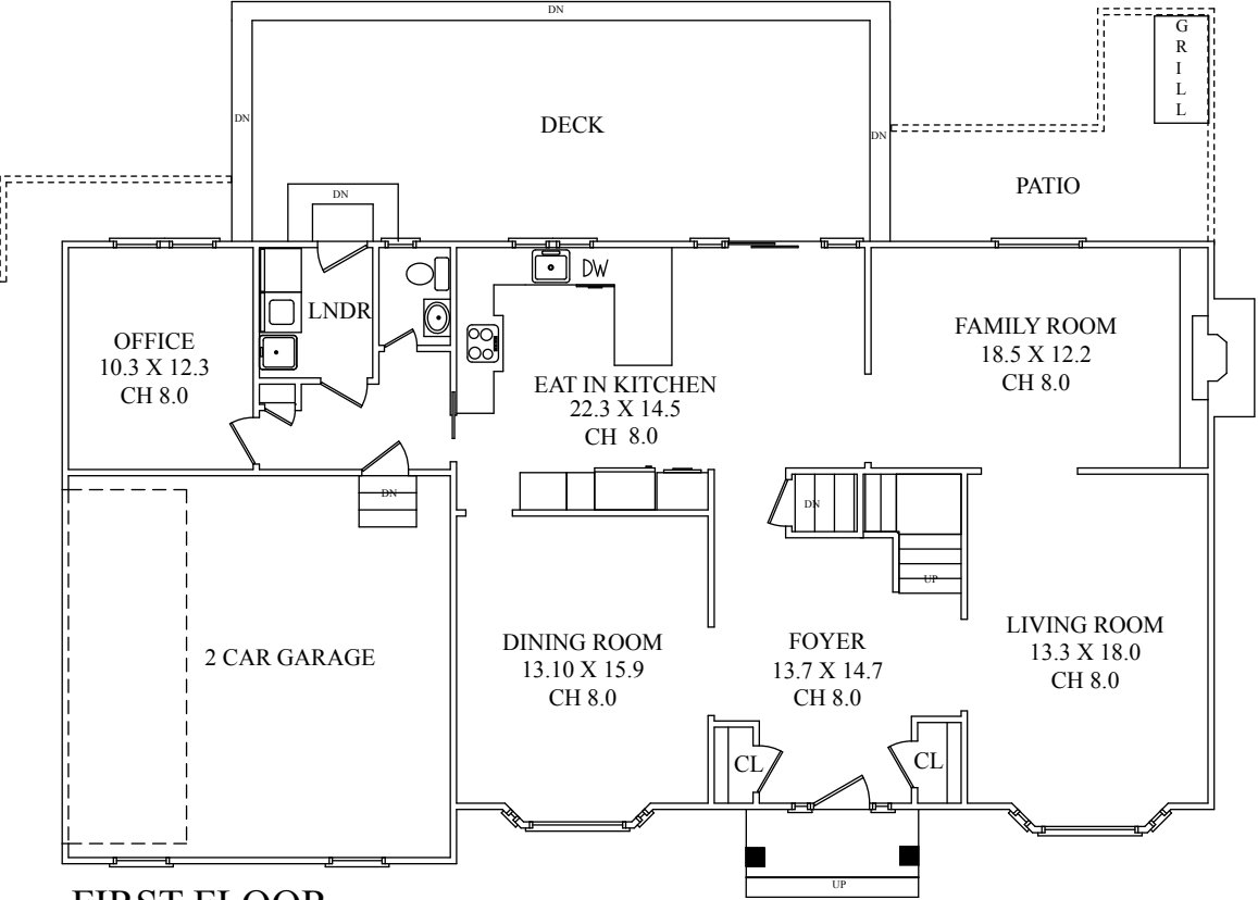
FIRST FLOOR
