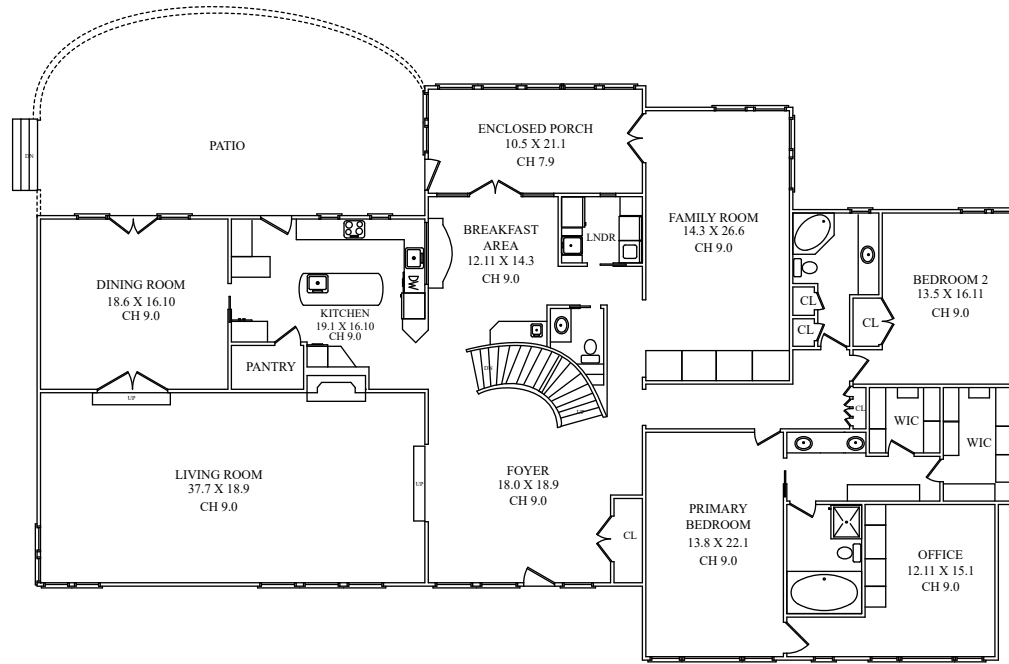
FIRST FLOOR
