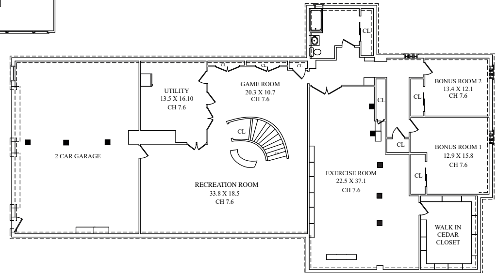
LOWER LEVEL
