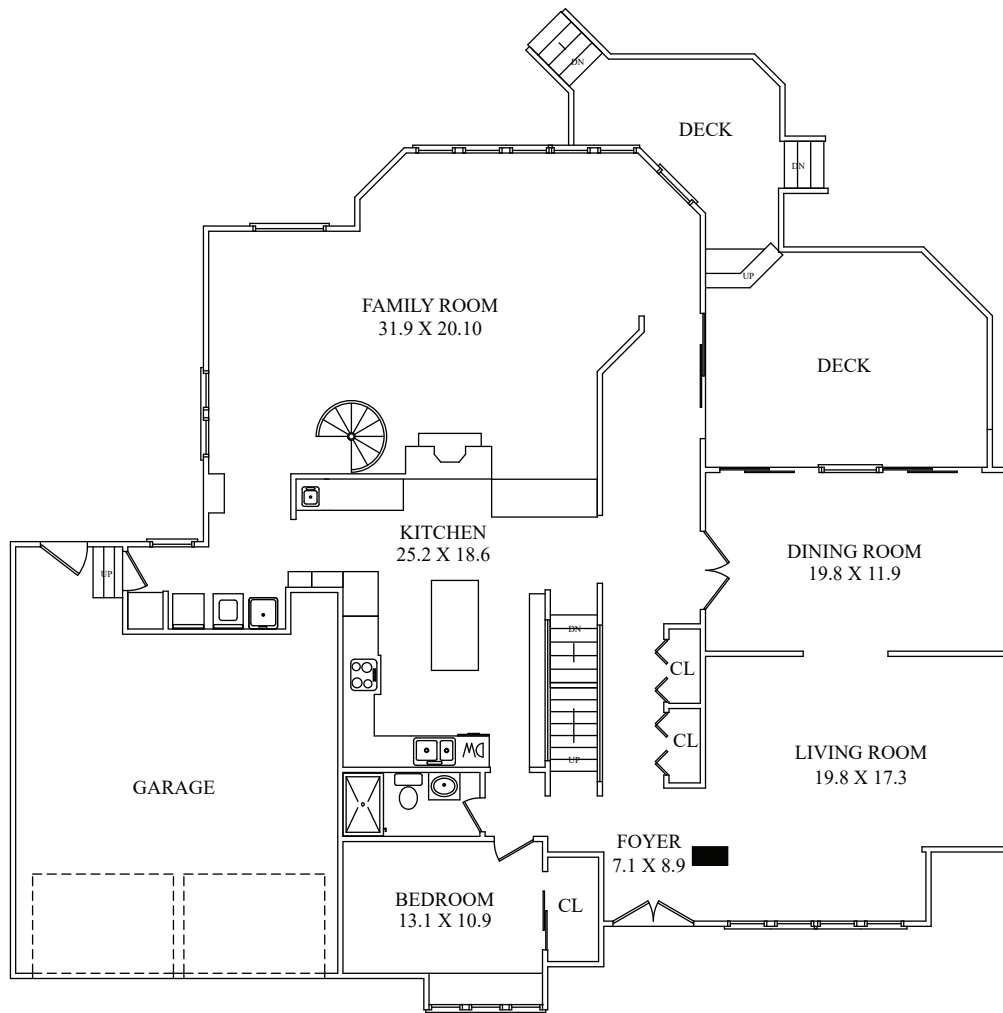
FIRST FLOOR
