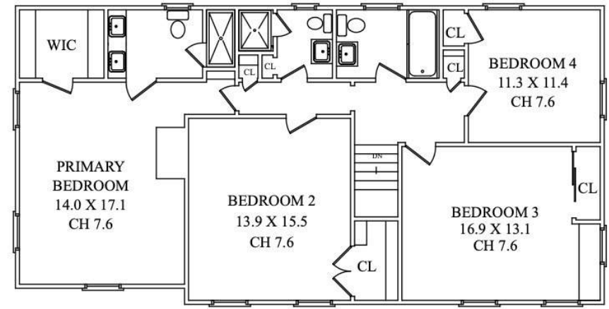
SECOND FLOOR 1187 SQFT
